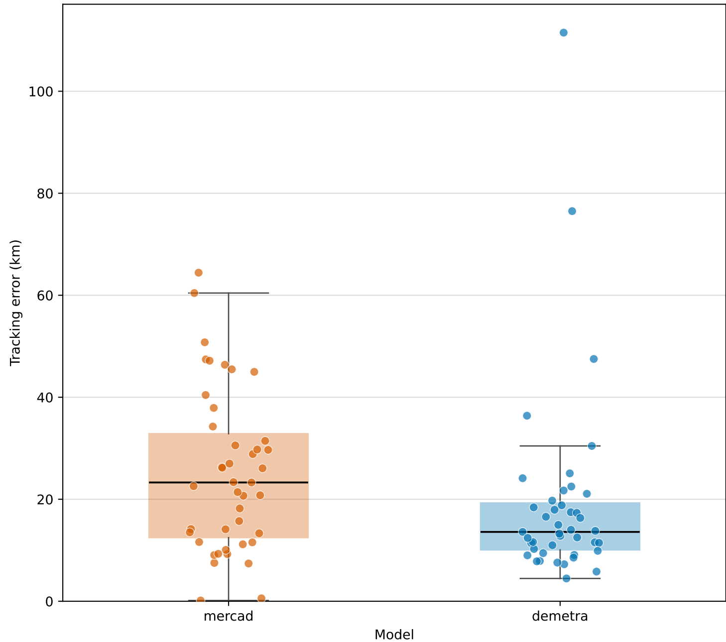
Distribution of cyclone-centre tracking errors relative to Manos
