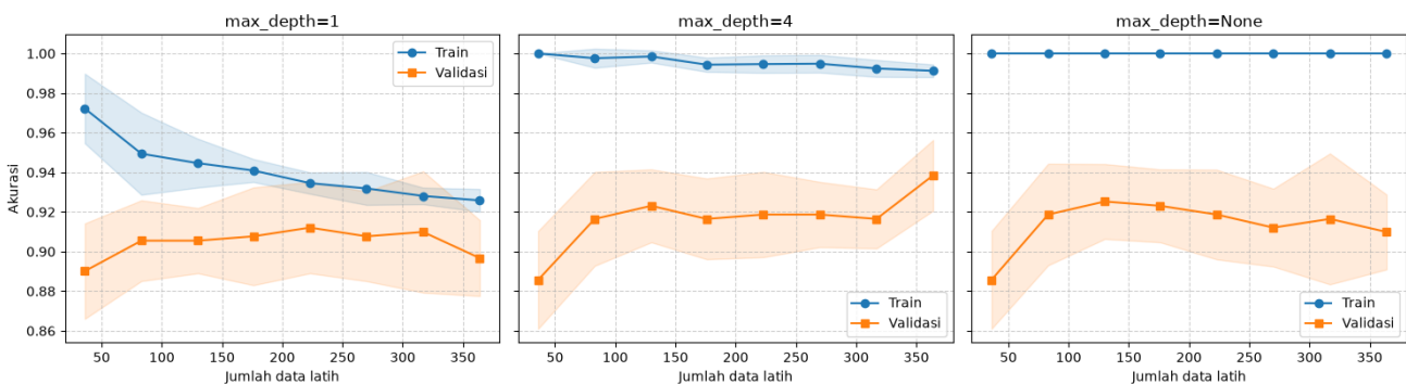
Learning Curve per max_depth — Decision Tree
