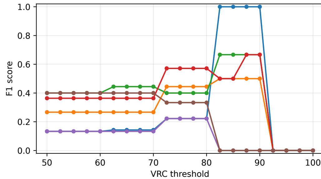
Relevant Functions
