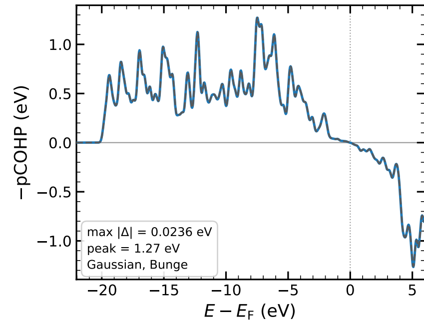
C nanotube, mean of 48 C-C
