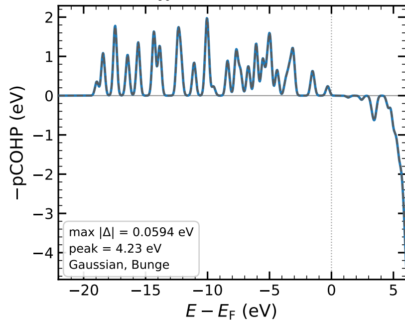
C 60 , mean of 90 C-C
