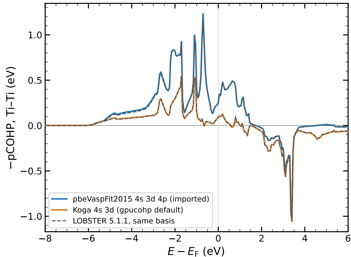
hcp Ti, 2.86 Å bond: -pCOHP
