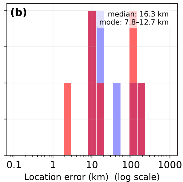
Uniform
