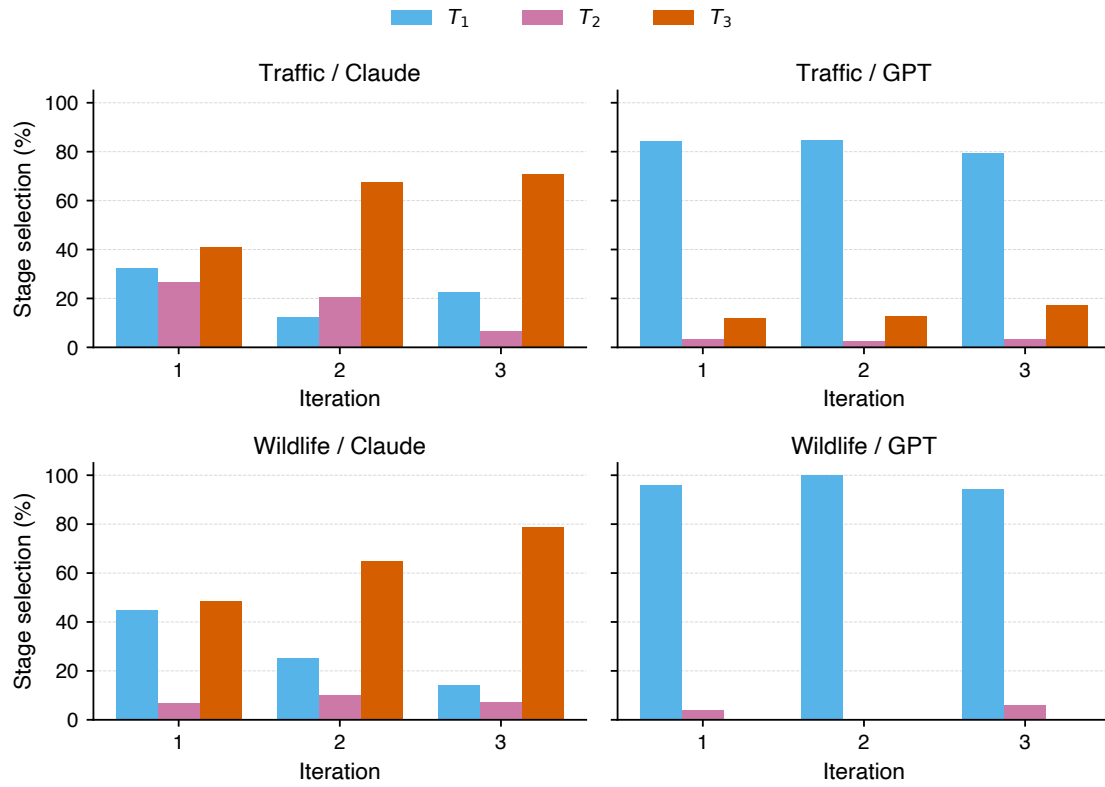
Figure 5: Per-iteration stage selection (Full condition) for each domain-model pair. Claude shifts toward T_3 in later iterations on both domains. GPT diagnoses T_1 at every iteration on both domains.
