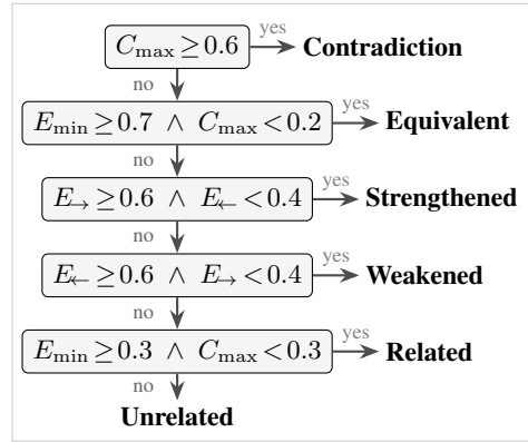
Figure 3: NLI diagnostic decision tree (first match wins). Thresholds are conservative. Equivalent demands strong bidirectional entailment ( \geq 0.7 ) with near-zero contradiction ( < 0.2 ), while Contradiction requires high conflict ( \geq 0.6 ).
