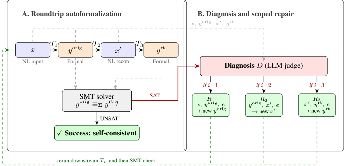
Figure 2: The roundtrip autoformalization framework. (A) The pipeline produces two formal encodings of x and an SMT solver checks them for equivalence. (B) On disagreement, diagnosis D localizes the failed stage and repair operator R_i corrects it before re-checking.
