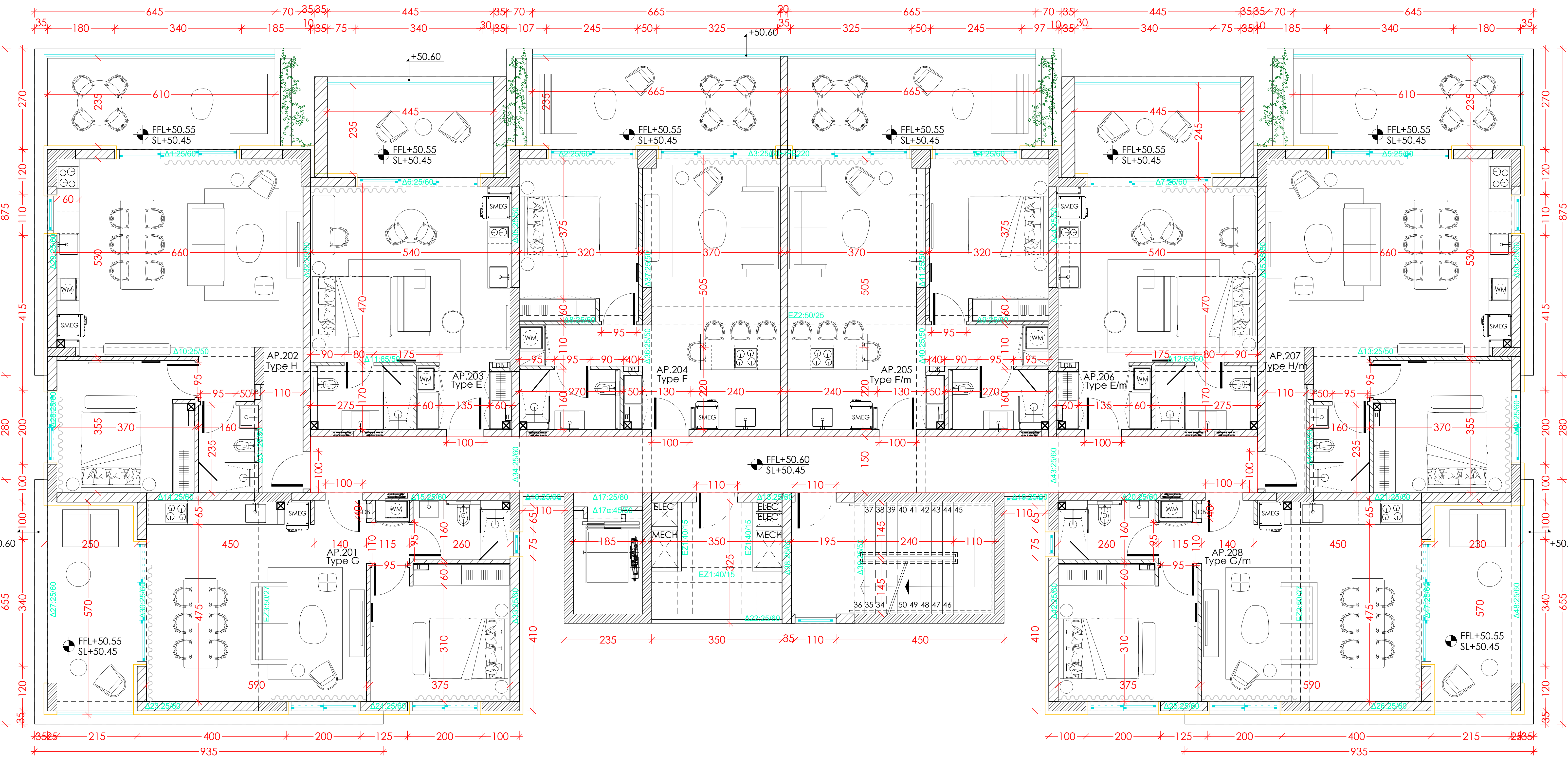
Building A second floor
