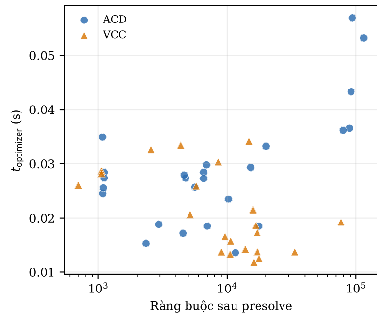
Spearman \rho = -0.047 ; p = 0.75
