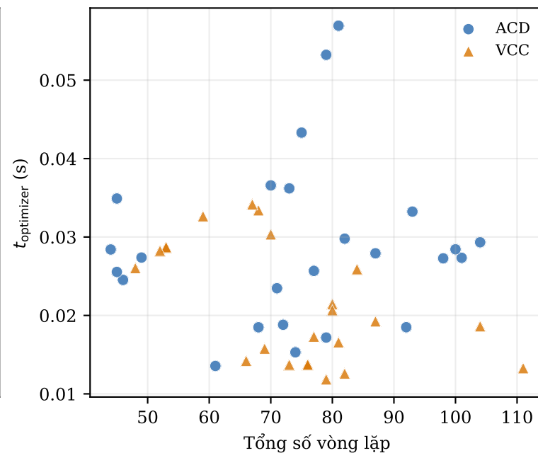
Spearman \rho = -0.150 ; p = 0.31
