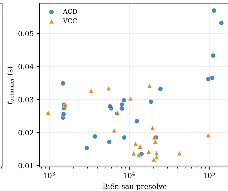
Spearman \rho = -0.043 ; p = 0.77
