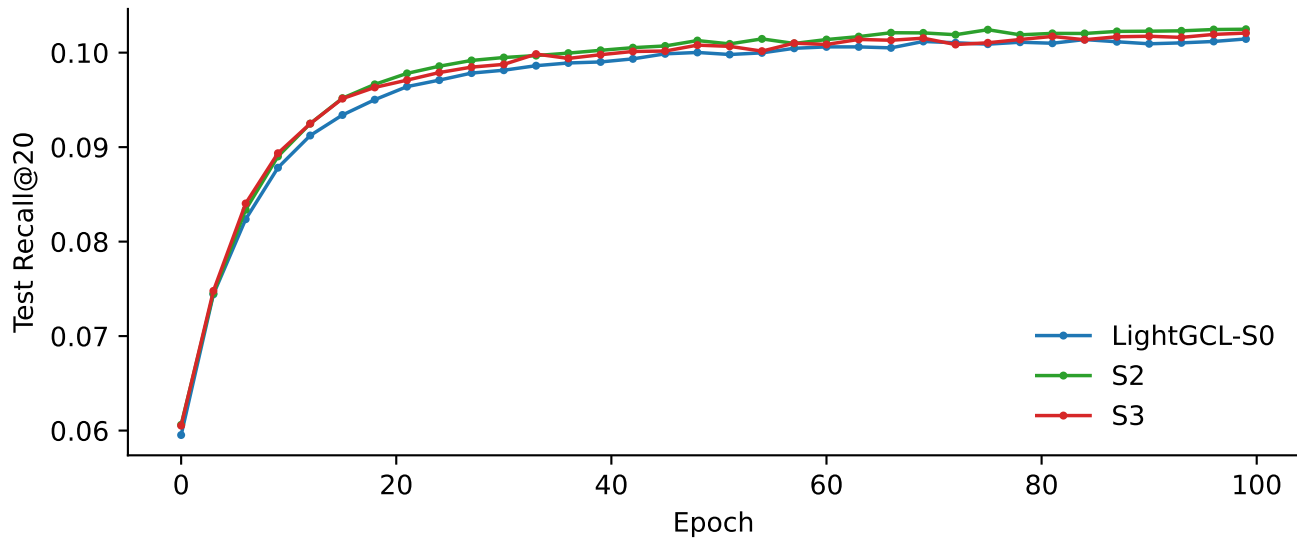
Test Recall@20 vs. epoch (seed 1)
