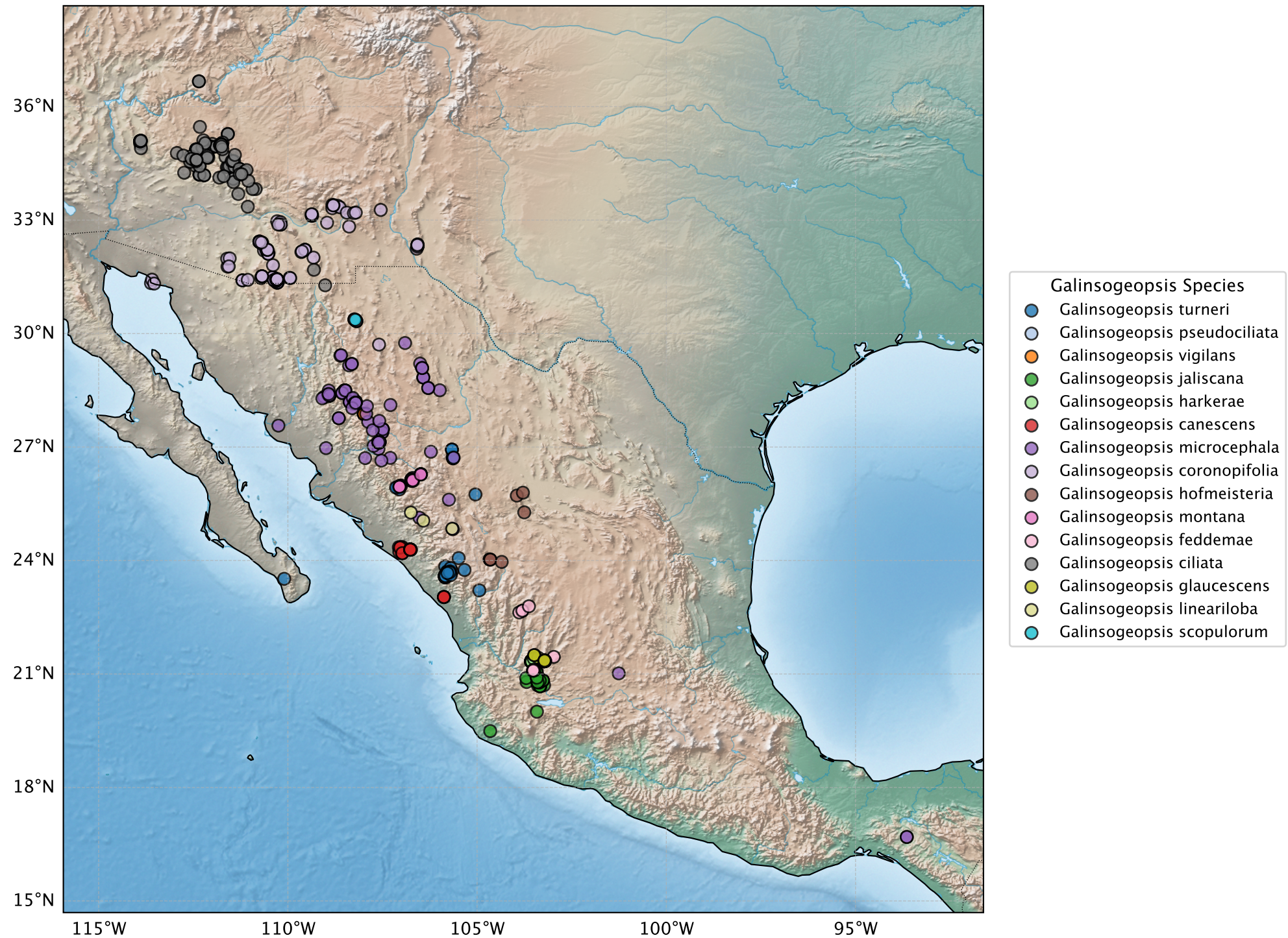
Geographical Positions by Galinsogeopsis Species
