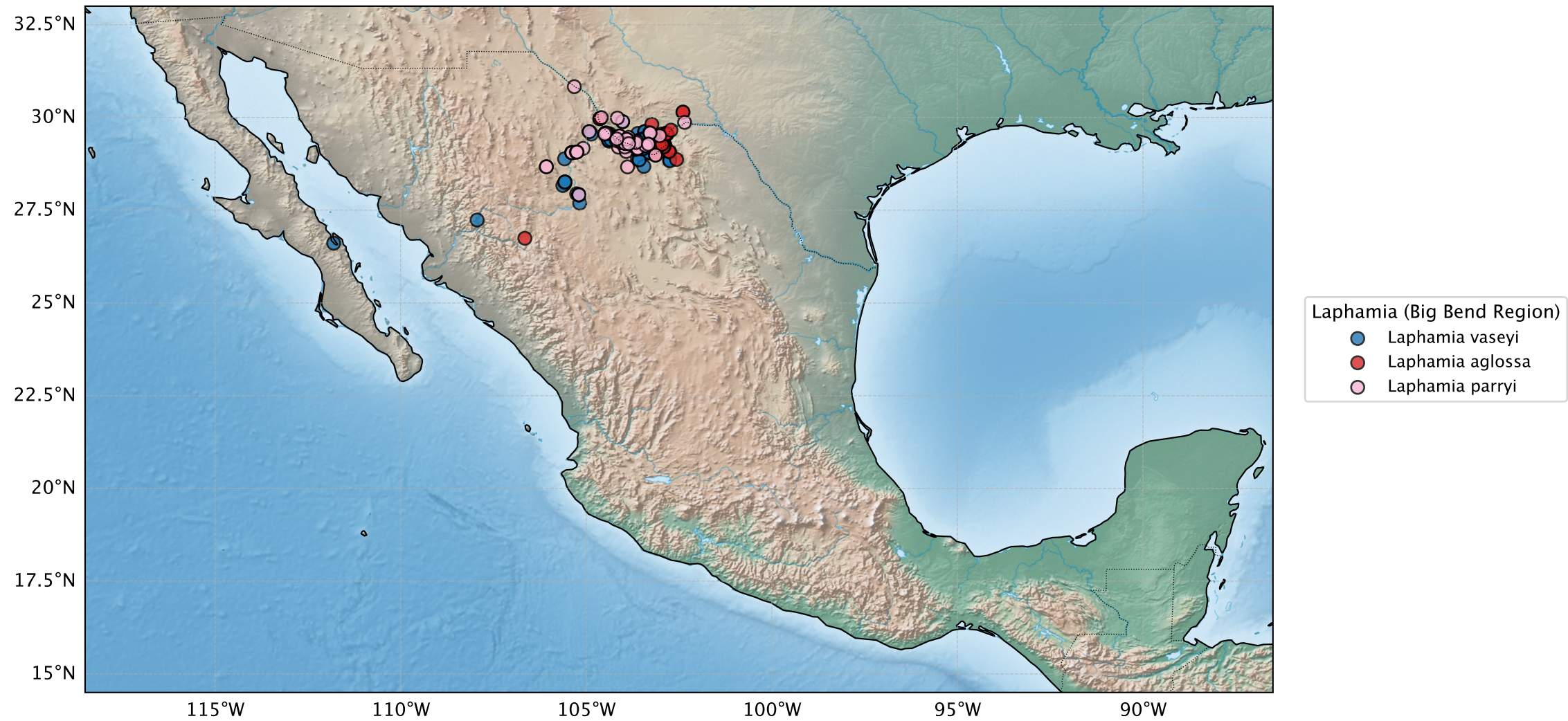
Geographical Positions by Laphamia (Big Bend Region)
