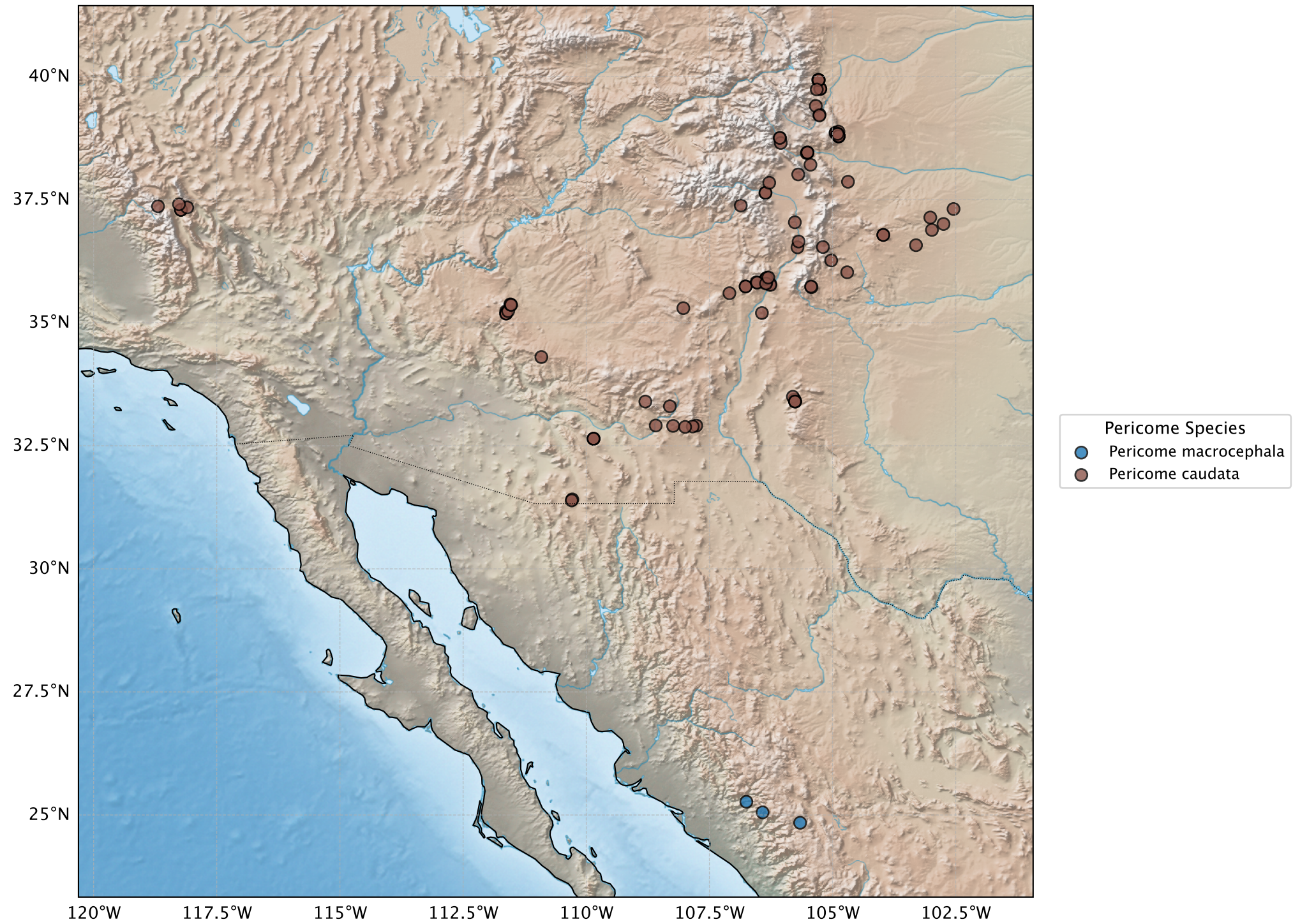
Geographical Positions by Pericome Species
