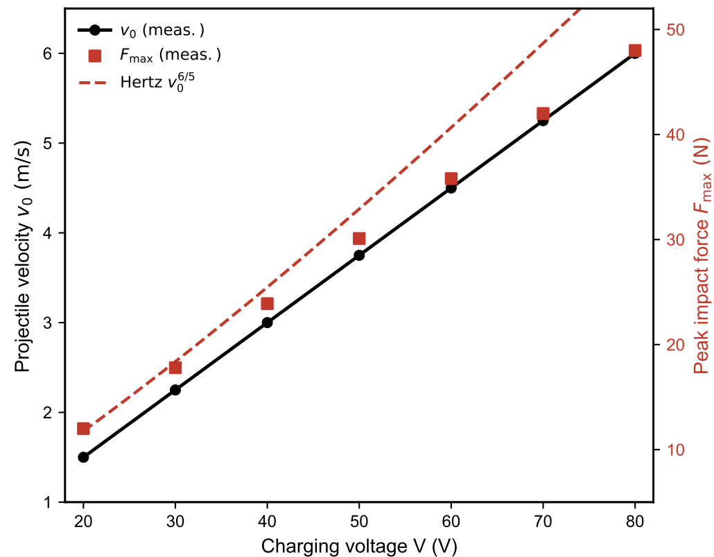
(b) v_0 and F_{\max} vs. voltage
