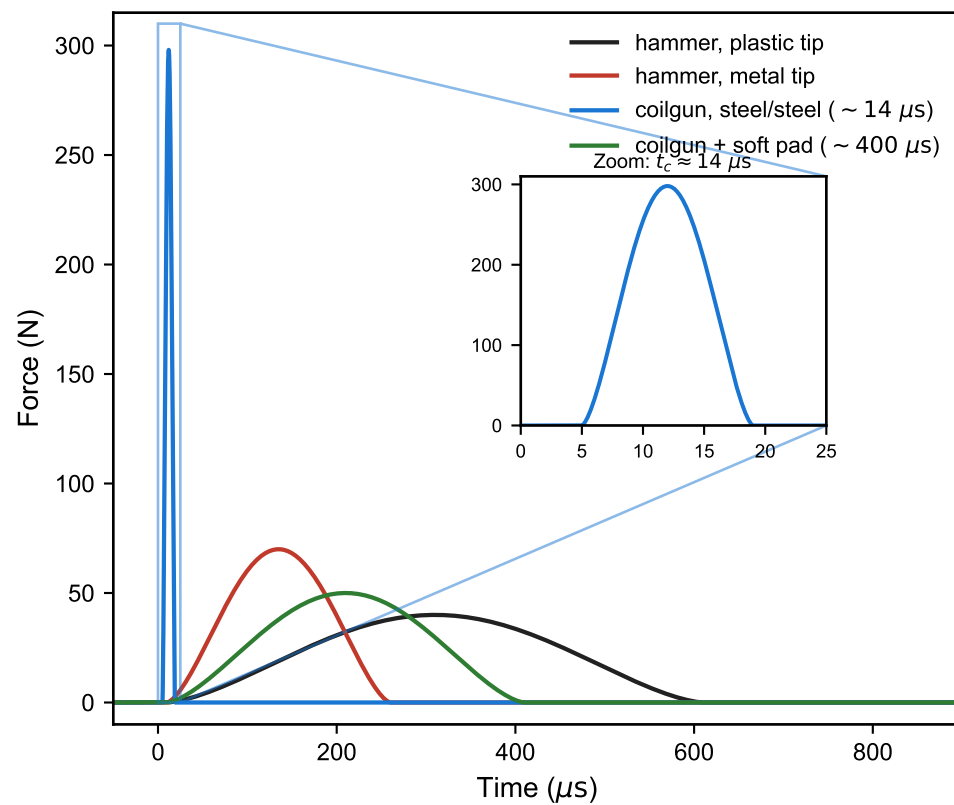
(c) Force histories
