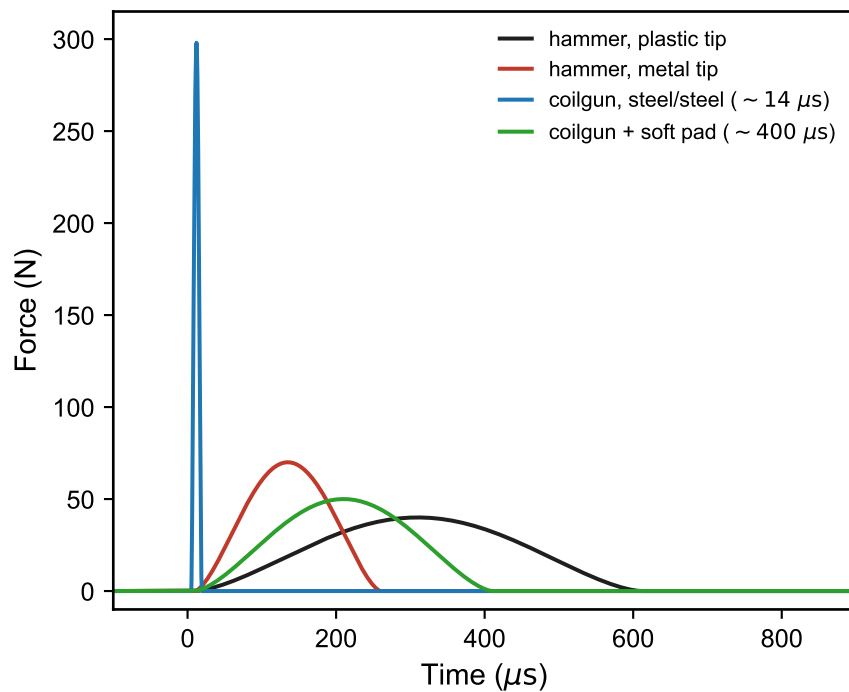
(c) Force histories
