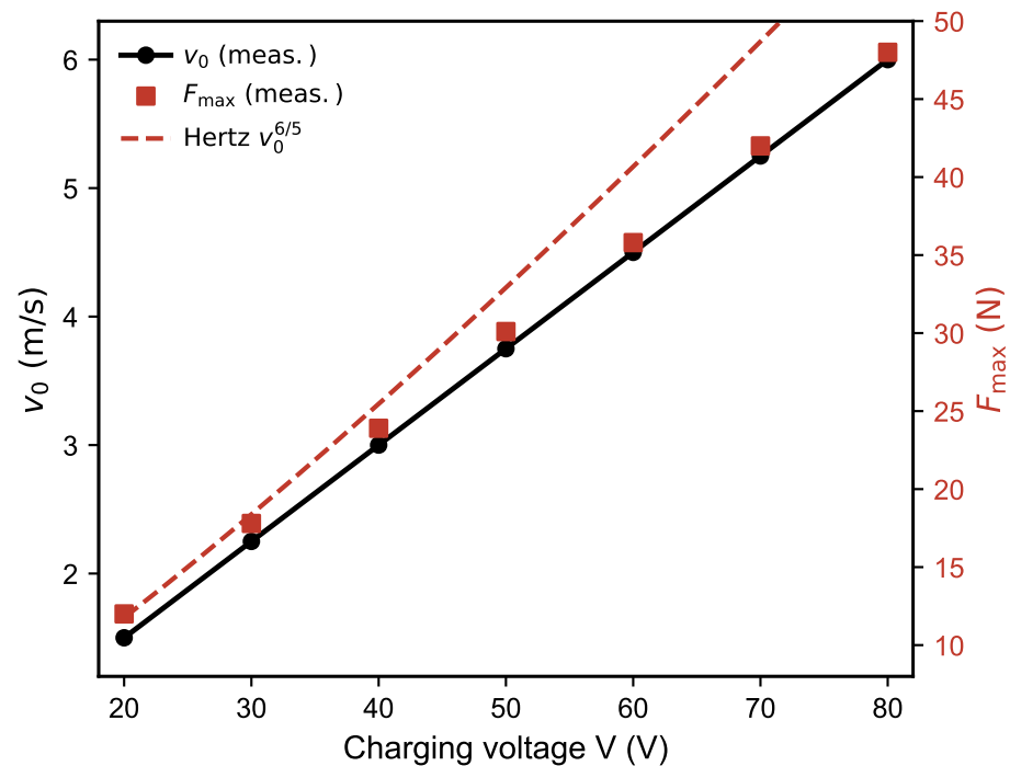
(b) v_0 and F_{\max} vs. voltage
