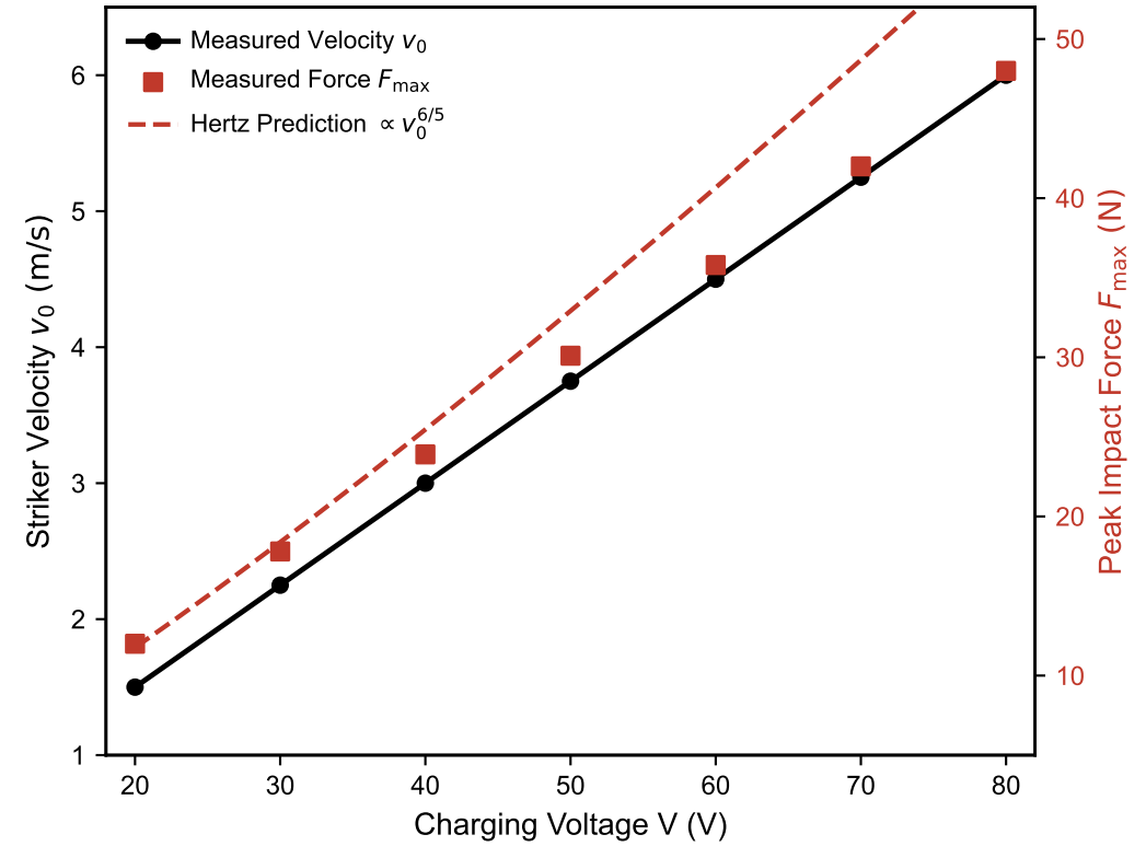
(b) Striker Velocity v_0 and Peak Force F_{\max} vs. Charging Voltage V
