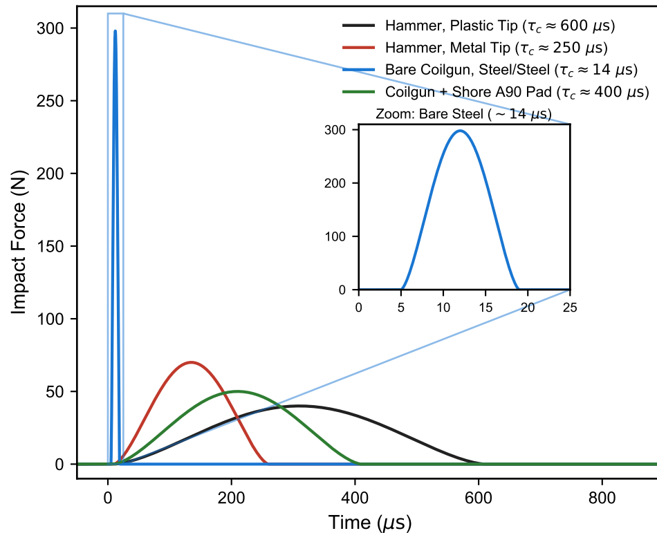
(c) Time-Domain Force Histories for Different Impactor Configurations
