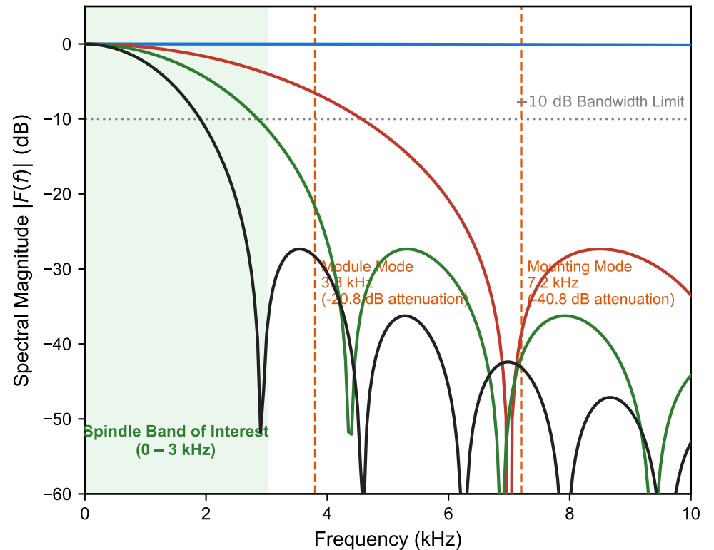
(d) Force Spectra & Mechanical Low-Pass Filtering of Parasitic Modes
