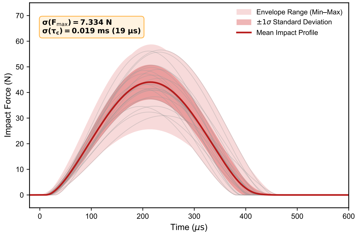
(a) Manual Impact Hammer (High Operator Dependency)
