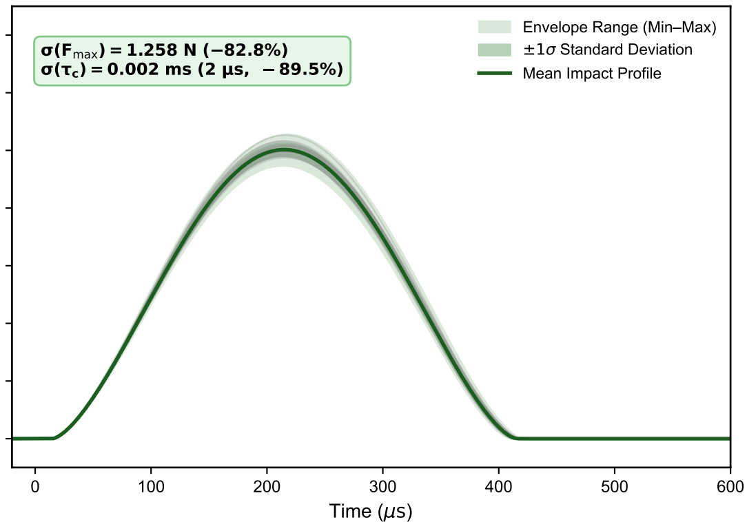
(b) Automated Gauss Exciter (Electronically Triggered Repeatability)
