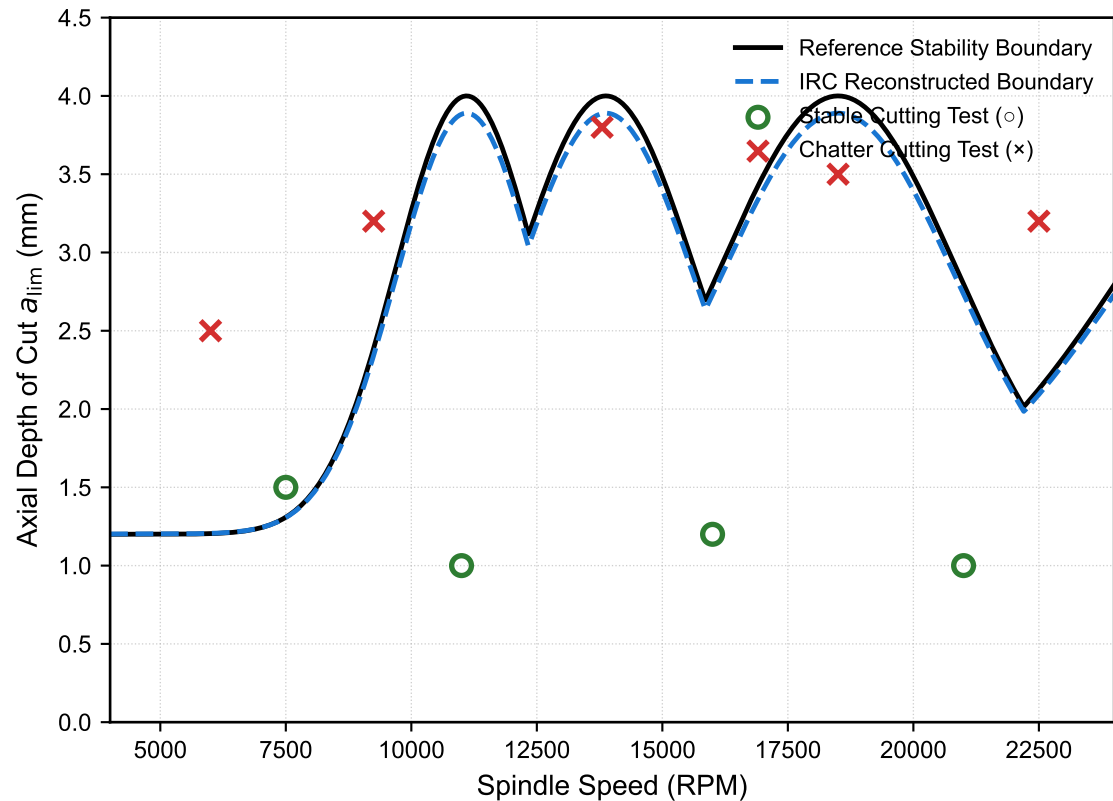
(b) Milling Stability Lobe Diagram (SLD) & Cutting Tests
