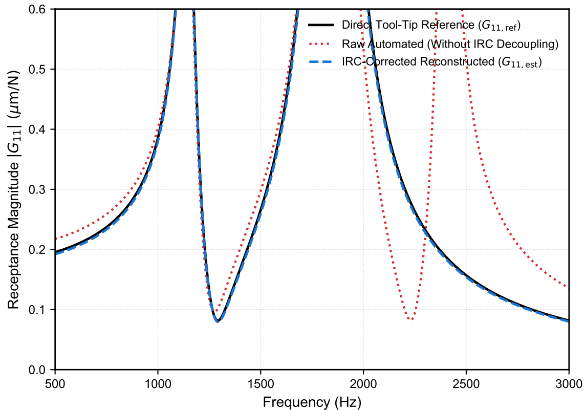
(a) Tool-Point FRF Magnitude |G_{11}(f)|
