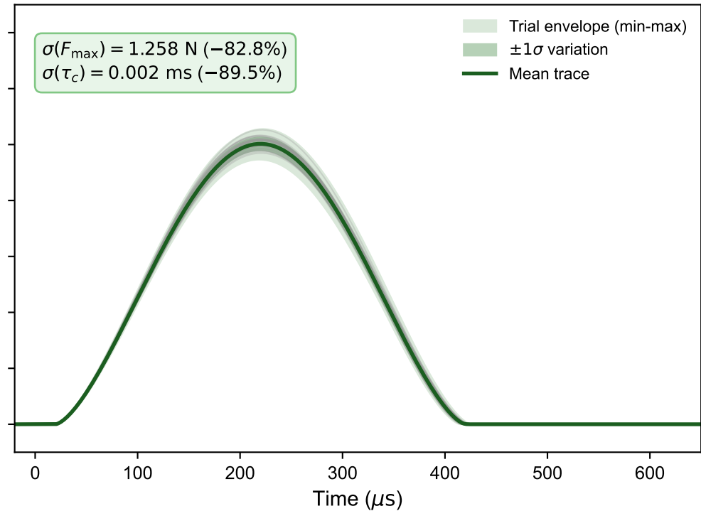
(b) Gauss exciter (100 trials)
