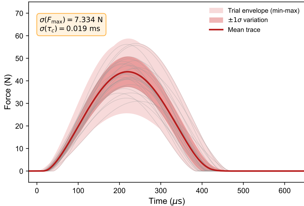
(a) Manual impact hammer (100 trials)
