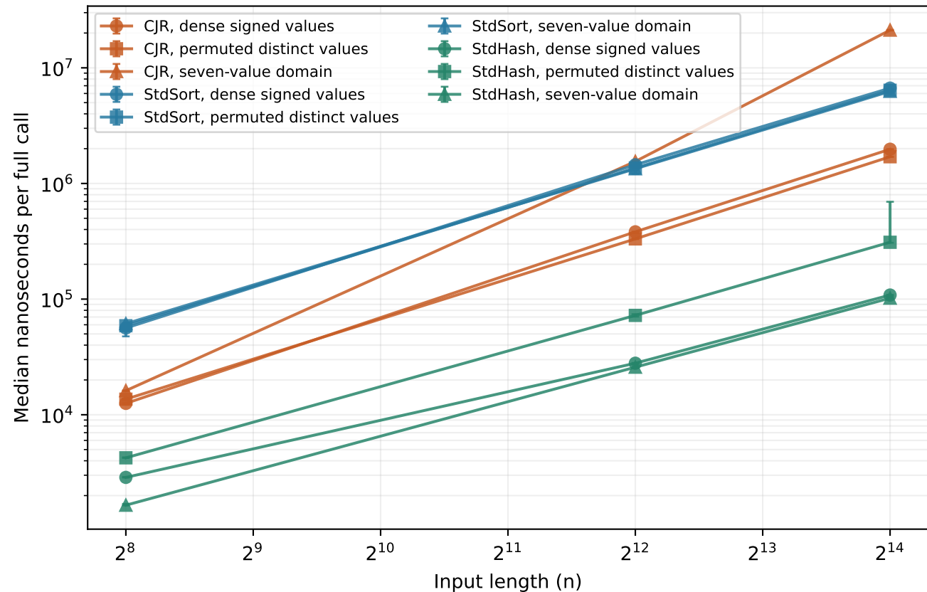
Scaling on three distributions
