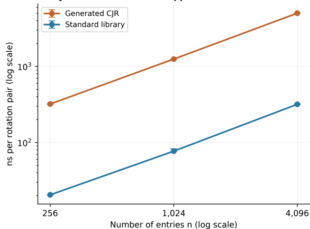
HashMap: hit, keys 1,000,000 to 1,000,000+ n-1
