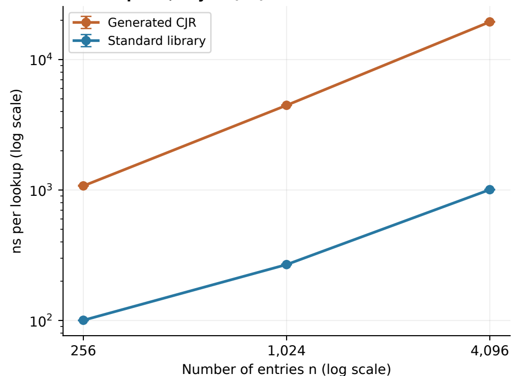
HashMap: hit, keys i \cdot (2n)
