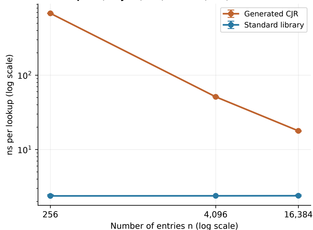
HashMap: hit, keys 1,000,000 to 1,000,000+ n-1
