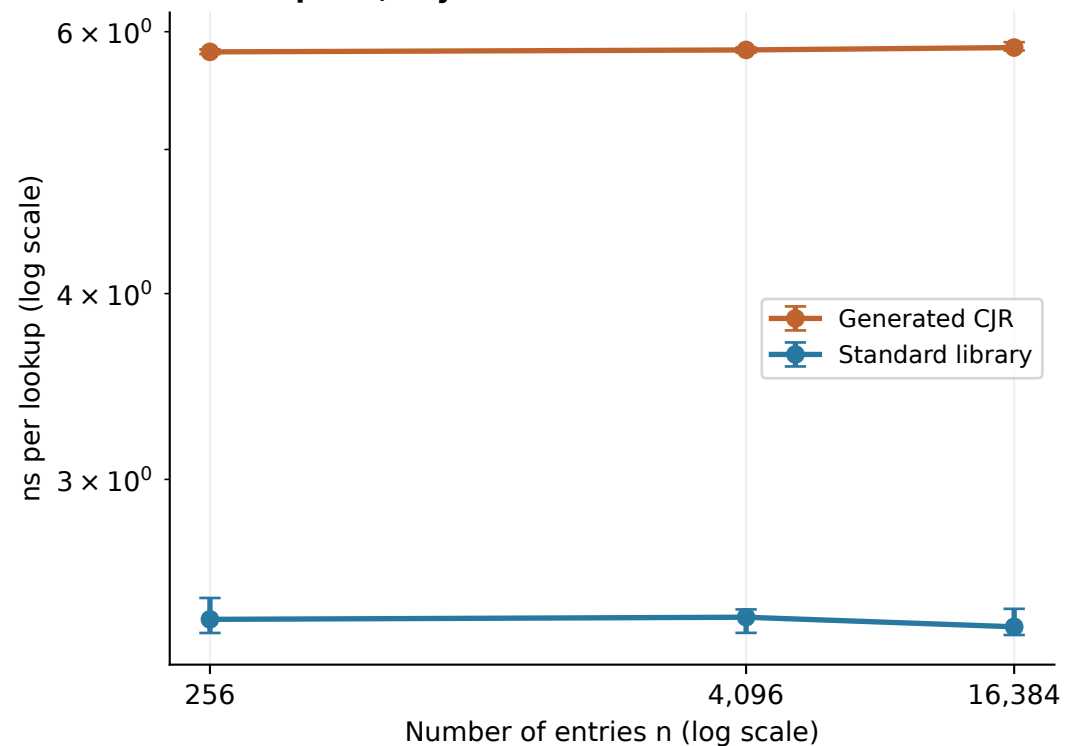
HashMap: hit, keys i \cdot (2n)
