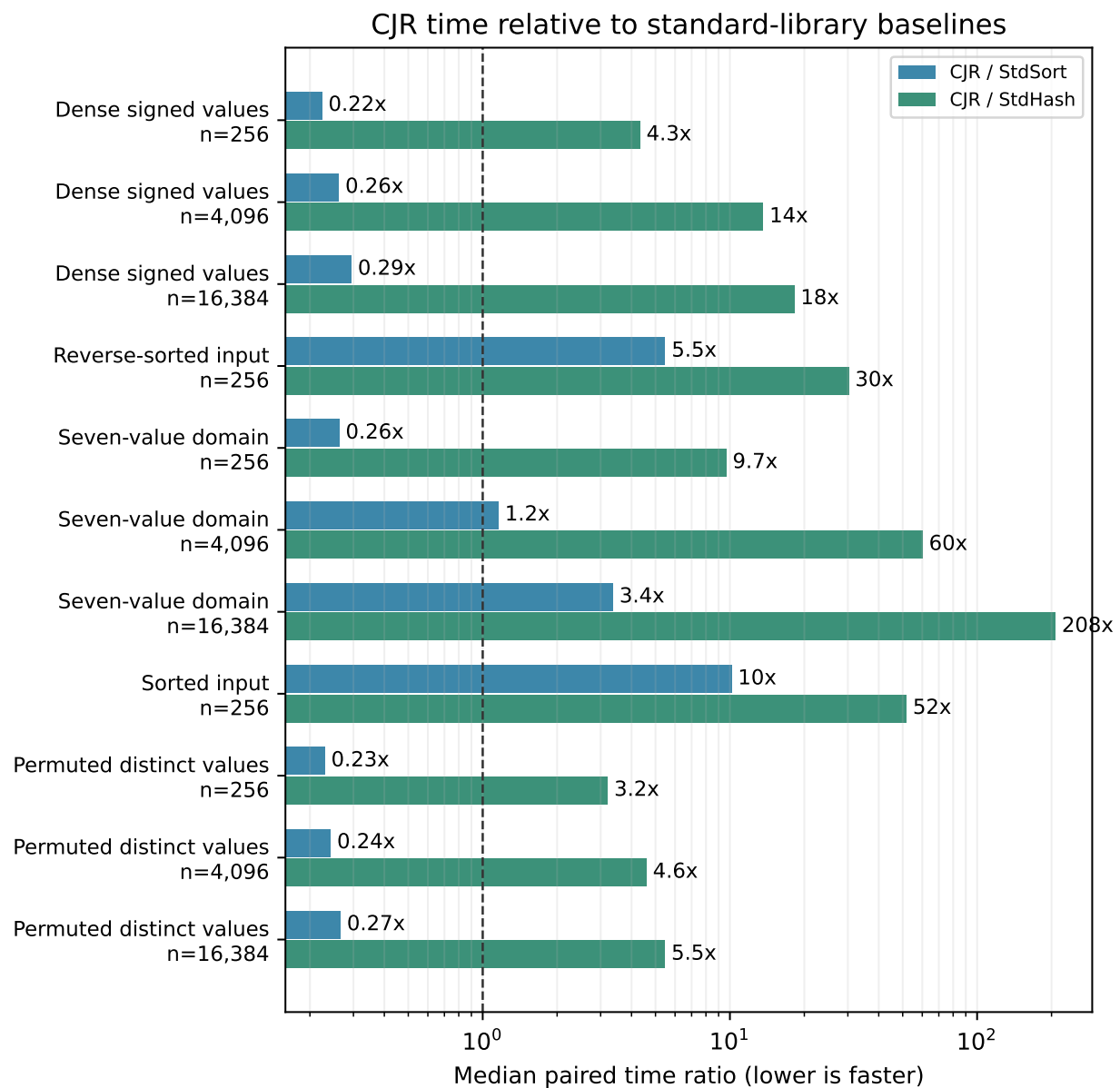
Figure 5: Median paired CJR/baseline ratios. Values above one mean CJR is slower.
