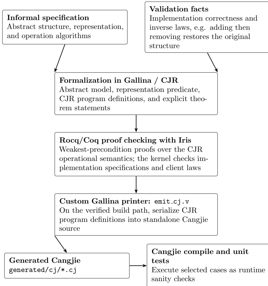
Figure 1: The intended specification-to-test workflow and the components implemented in this repository. The LLM-assisted formalization is a human review point; proof checking validates CJR theorems, while unit tests sample the separately printed Cangjie program.
