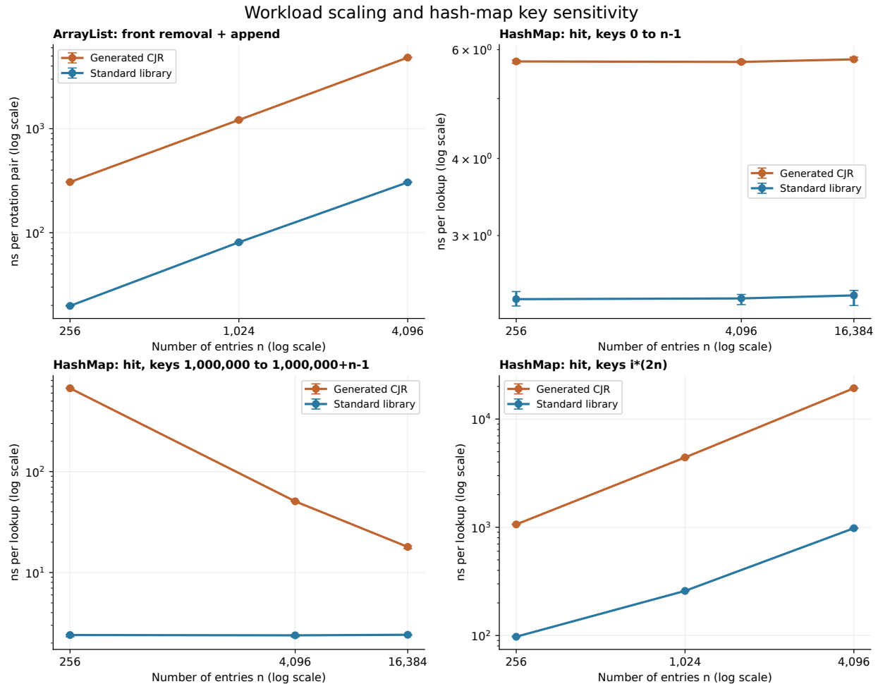
Figure 3: Scaling of front rotation and hash-map queries. Both axes use logarithmic scales. Lines show individual median times, with interquartile error whiskers. In the large-key case, the CJR time falls as capacity grows, because remainder normalization needs fewer subtractions. Colliding keys show increasing query costs for both implementations.
