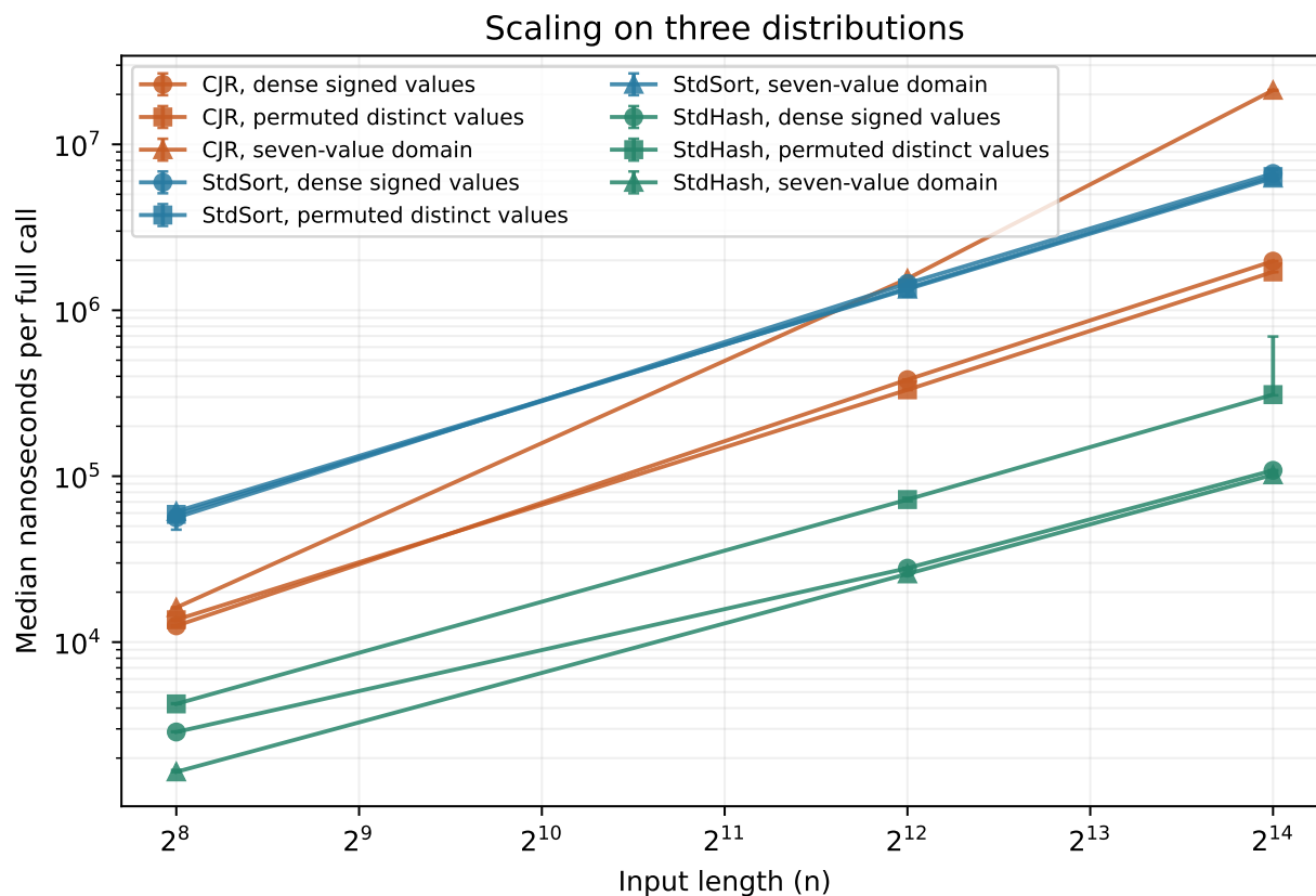
Figure 4: Complete-operation timings: median elapsed time per call; error bars show the interquartile range across 21 samples.
