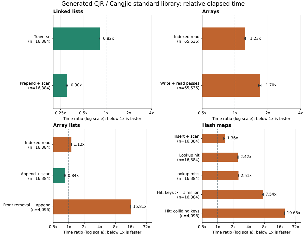
Figure 2: Relative elapsed time of generated CJR and standard-library workloads at their largest tested sizes. The dashed line is equal time; bars and error whiskers are the median and interquartile range of paired CJR/standard ratios. List build/scan, array-list build/scan, and map build/scan include construction and growth; the other setups are excluded.
