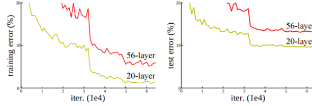
Figure 22: Training and Test Error Degradation
