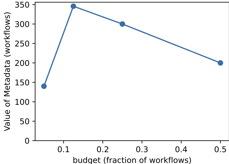
Leverage needs budget to spend
