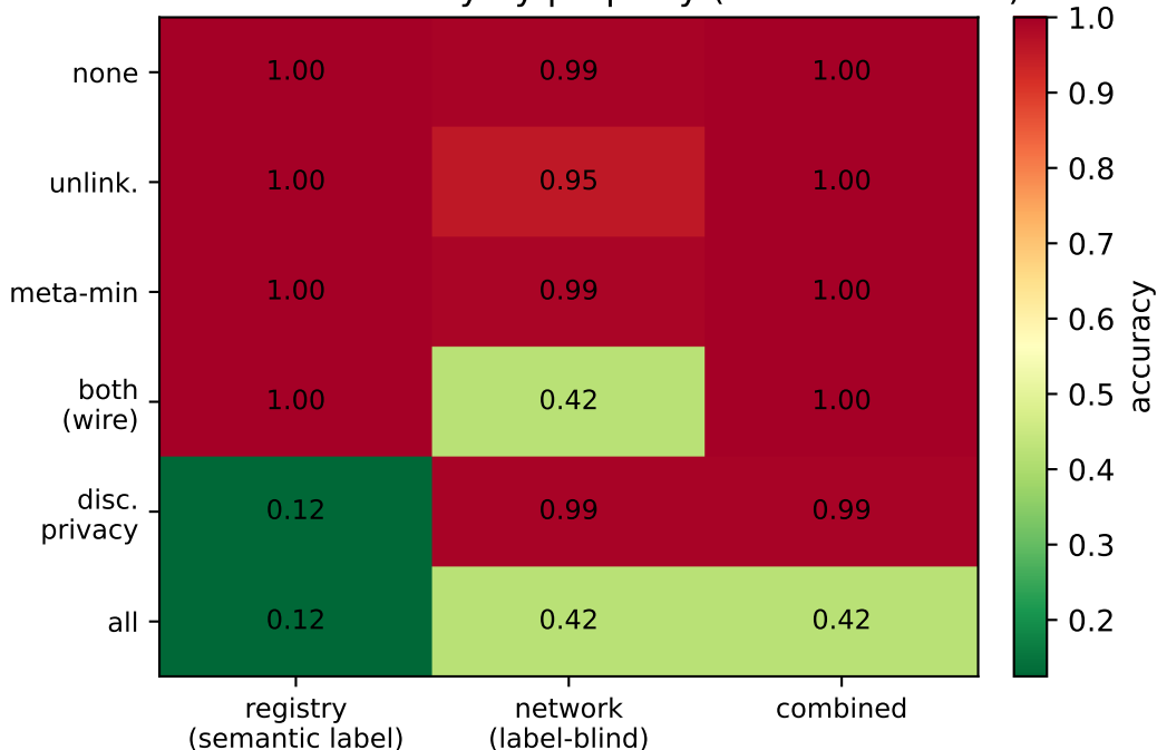
Protection: accuracy by property (chance = 0.125)
