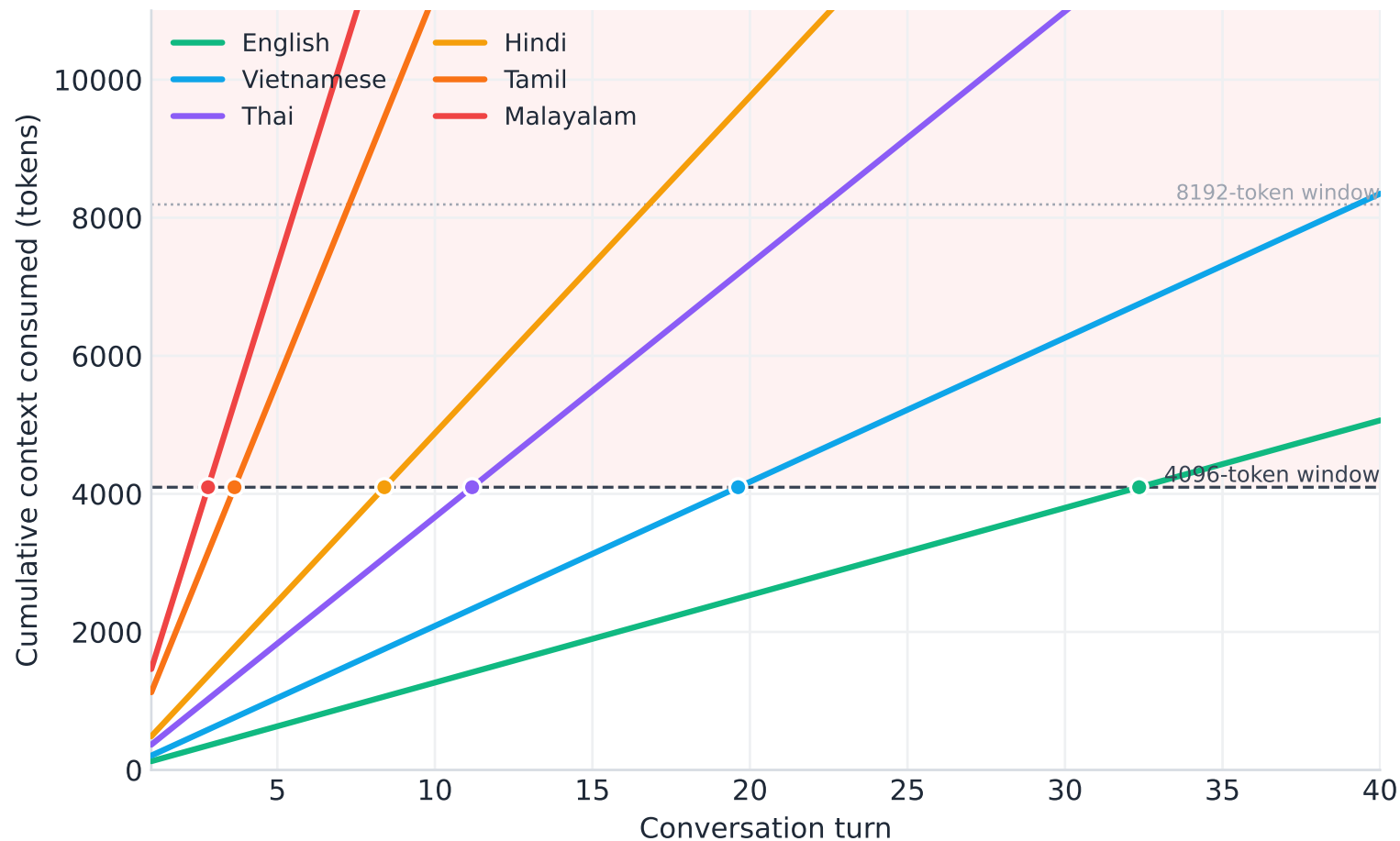
Figure 2. Context-window exhaustion rate by language (GPT-4/3.5 tokenizer)
