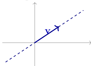
\text{span}\{\mathbf{v}\} = \text{đường}
