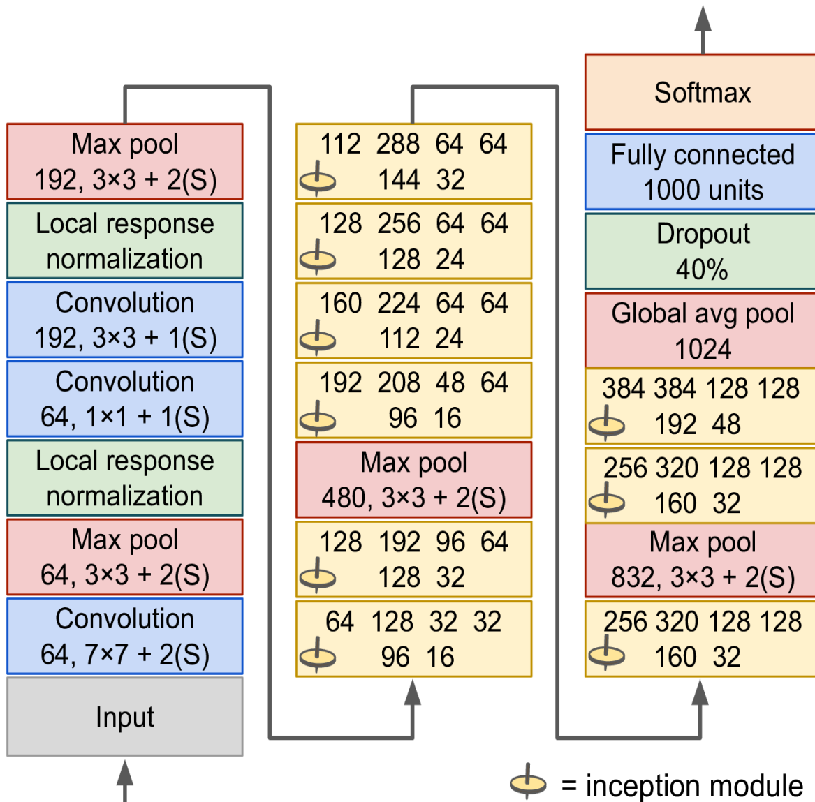
Figure 14-15. GoogLeNet architecture
