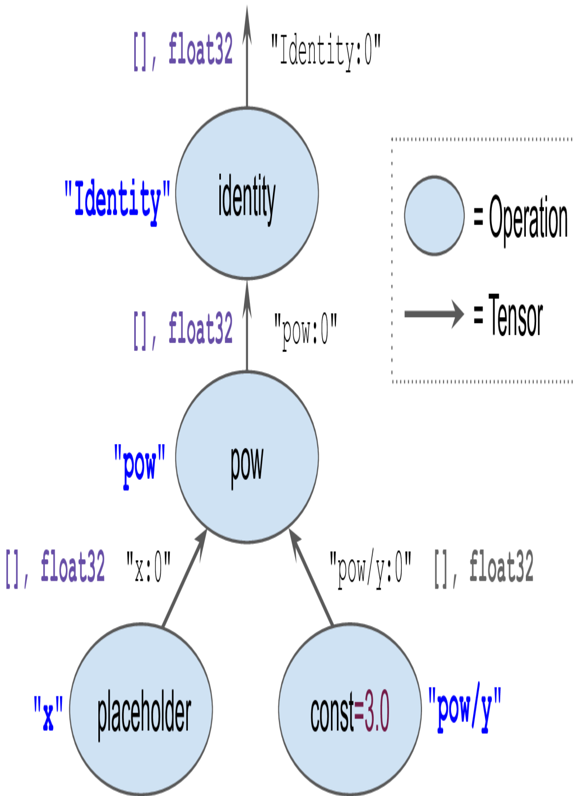
Figure D-2. Example of a computation graph
