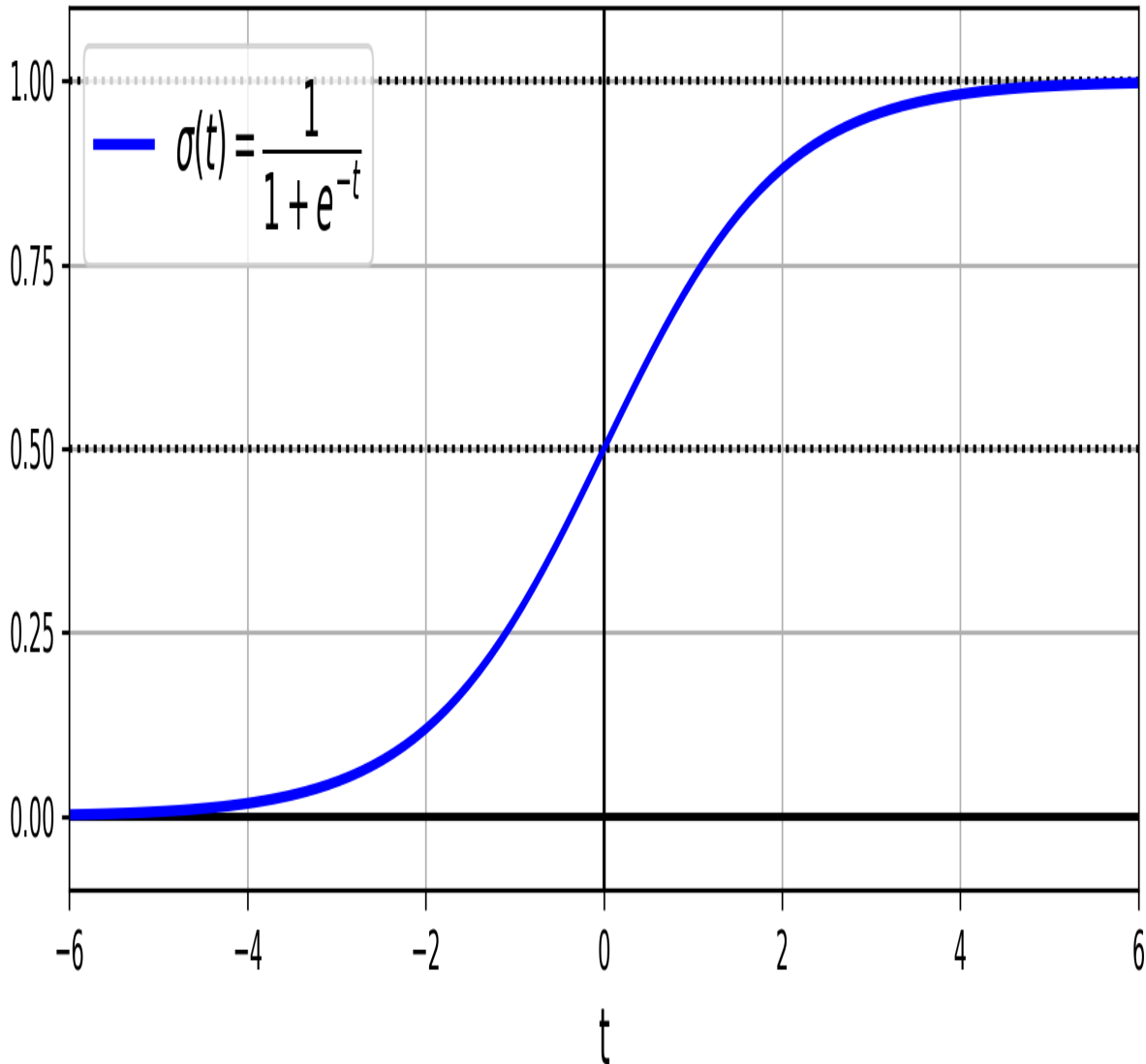
Figure 4-21. Logistic function
