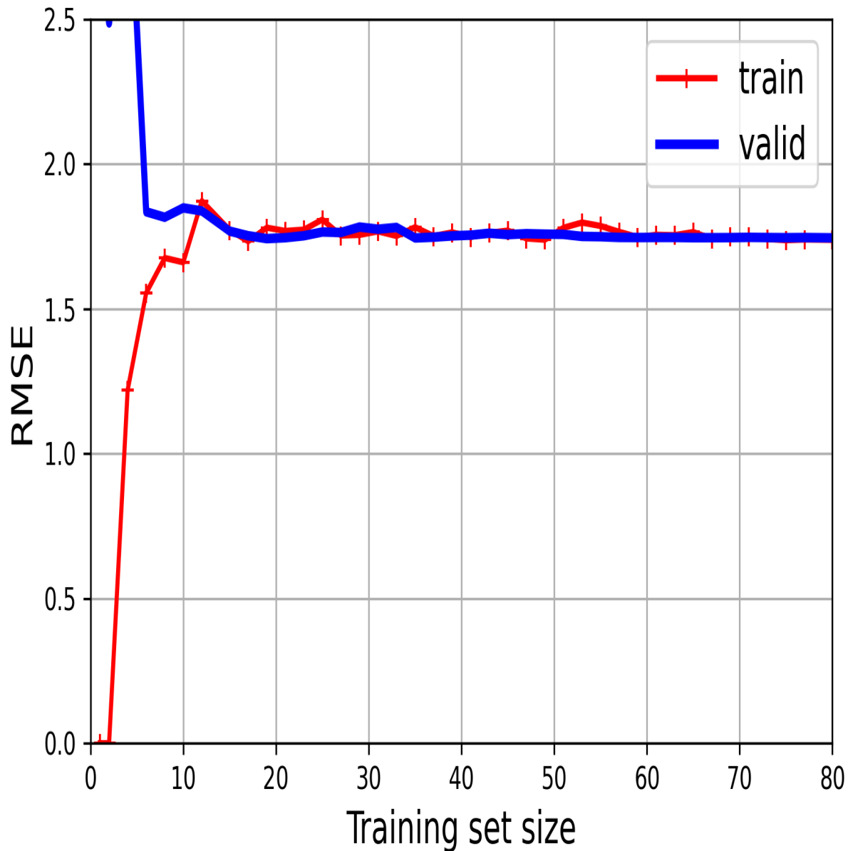
Figure 4-15. Learning curves
