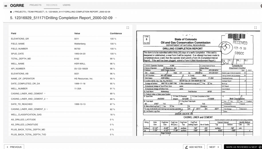
Figure 2: OGRRE UI. This screen shows review of a document. The fields on the left show extracted field-value pairs, which can be edited by a person and saved to the database. As fields are selected on the left, the corresponding bounding box detected by the AI processing are highlighted in the image on the right. Document review statuses can be set using buttons at the bottom of the page. Numerous keyboard shortcuts allow for navigation through a list of documents.
