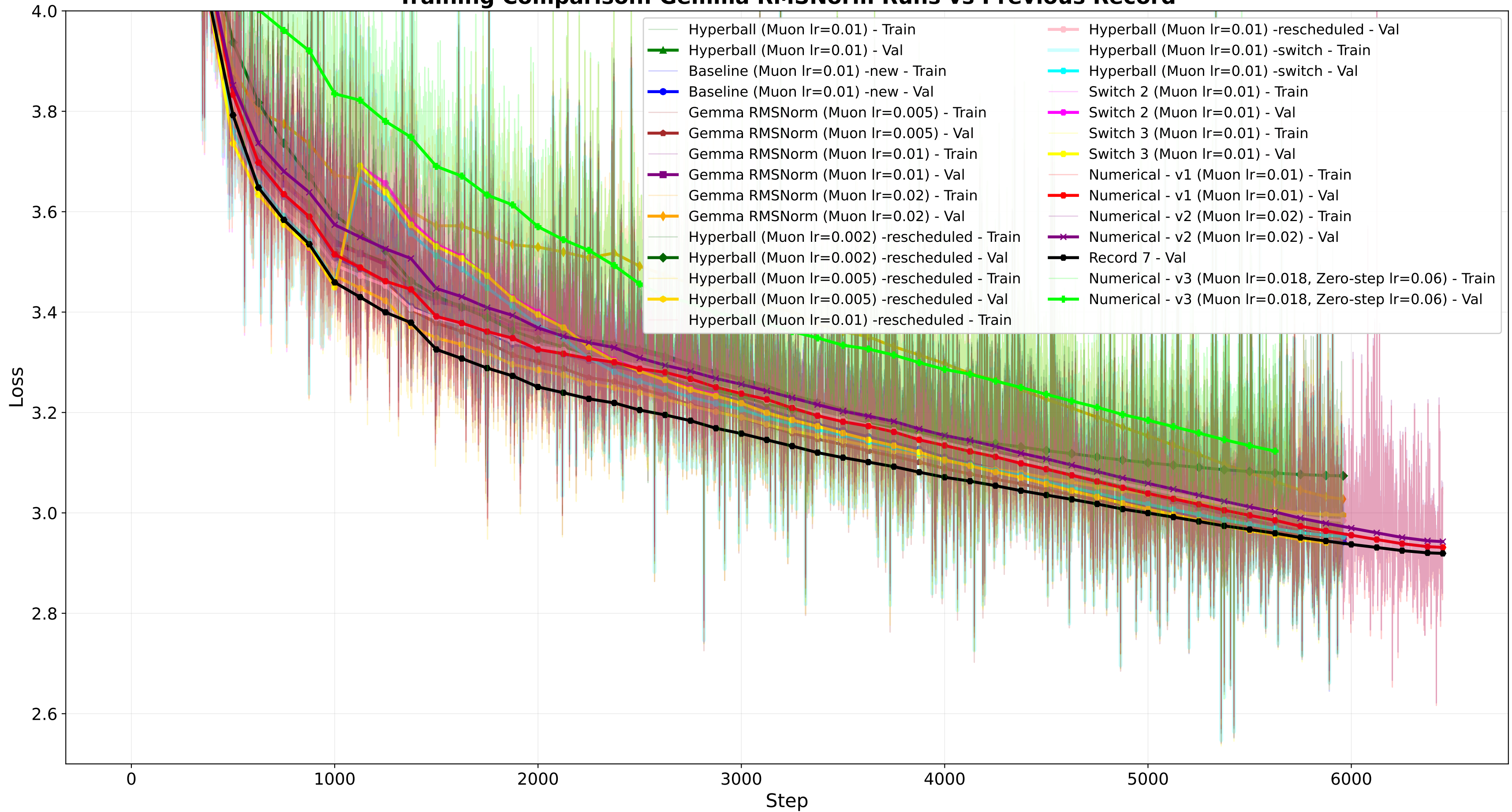
Training Comparison: Gemma RMSNorm Runs vs Previous Record
