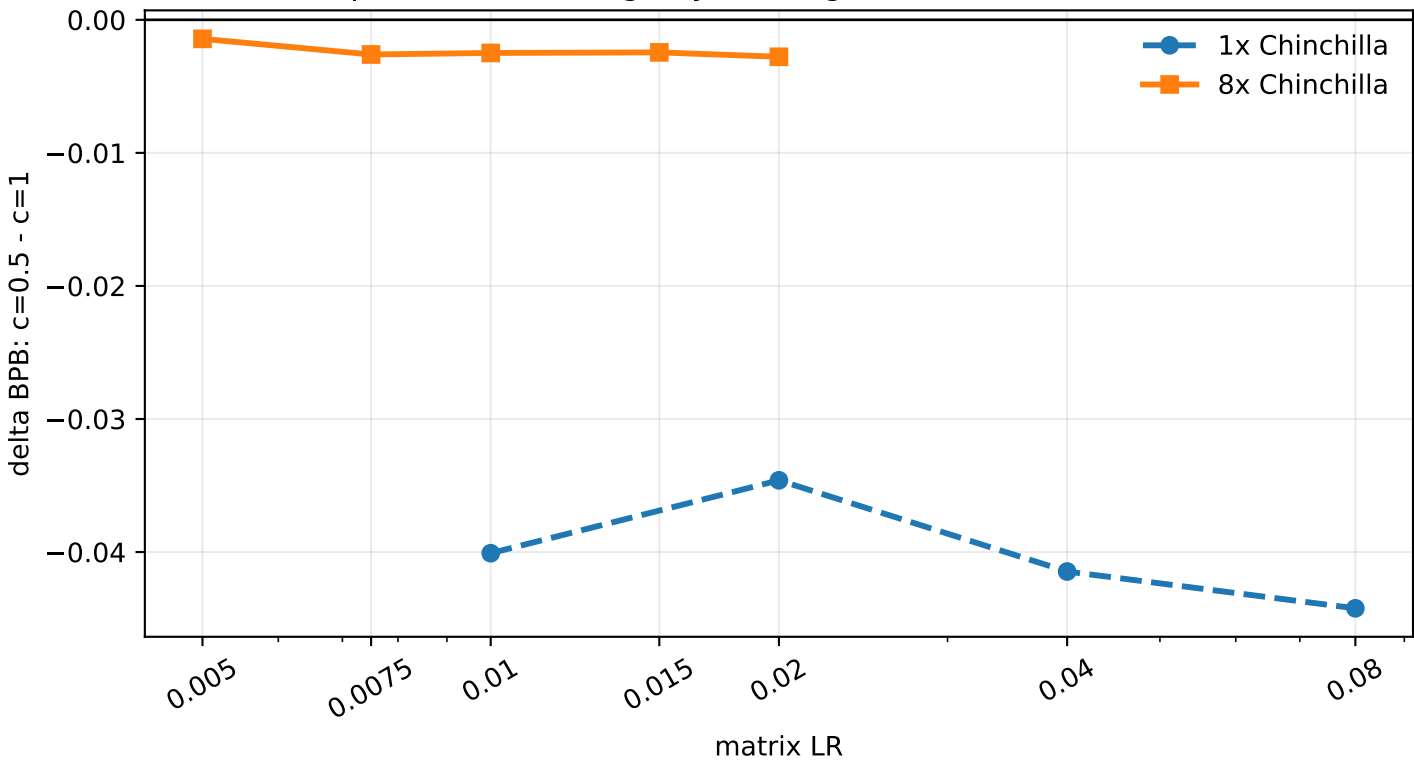
Top-Aware advantage by LR (negative means c=0.5 wins)
