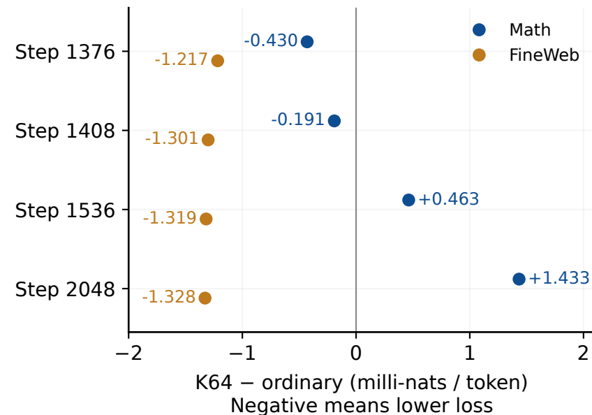
C Fixed LR1e-5 contrasts
