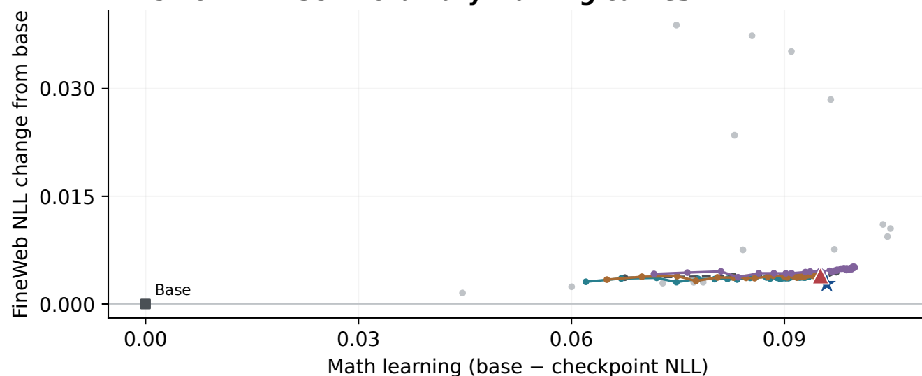
A SmolLM2-135M: ordinary training curves
