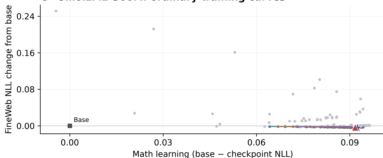
C SmolLM2-360M: ordinary training curves
