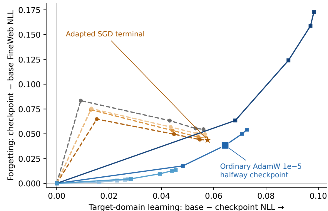
a Code · fixed quarter data, four passes
