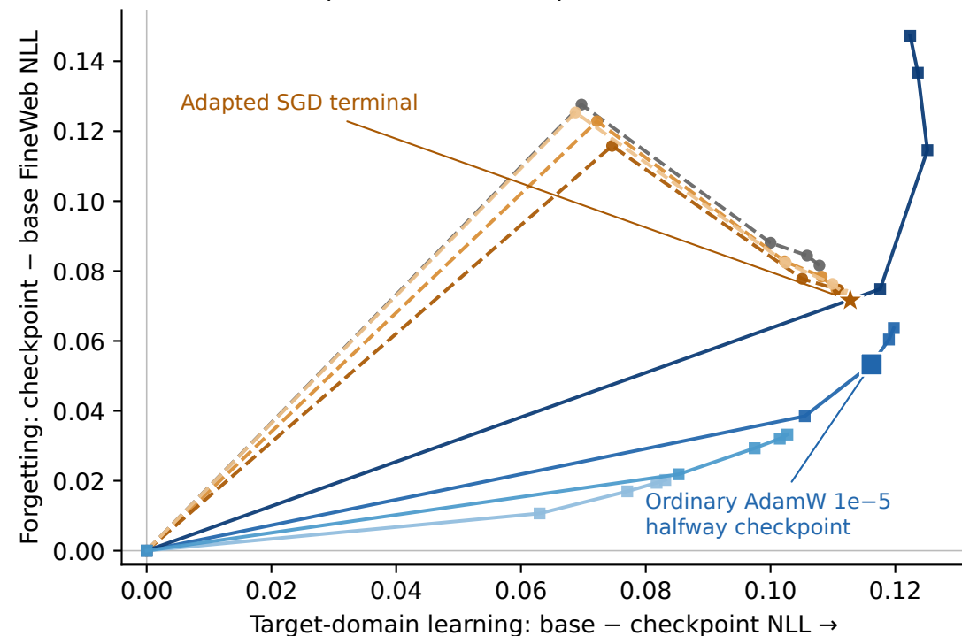
b Math · fixed quarter data, four passes
