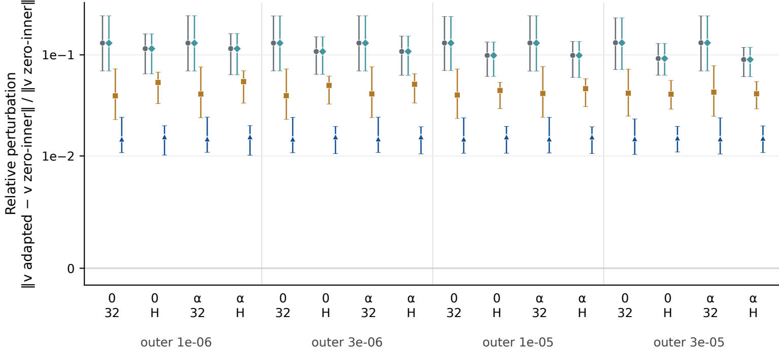
b Code · fixed quarter, four passes
