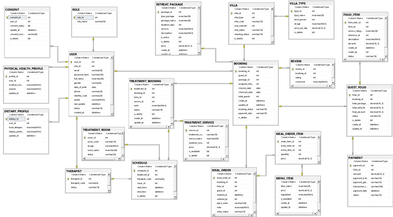
Figure X - Database Design Diagram
