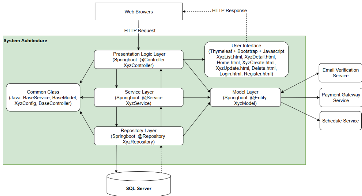
Figure X - Software Architecture
