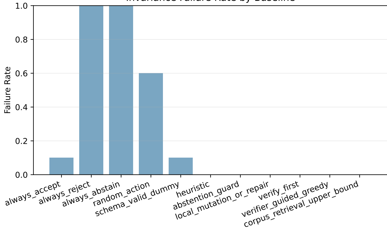
Invariance Failure Rate by Baseline
