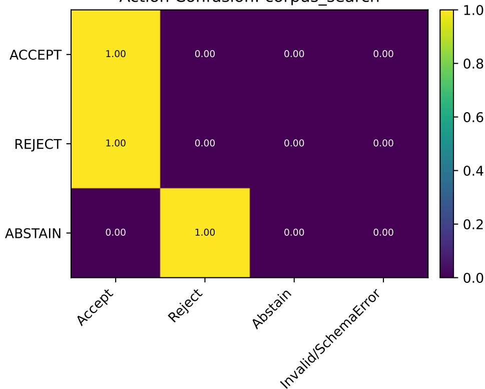
Action Confusion: corpus_search
