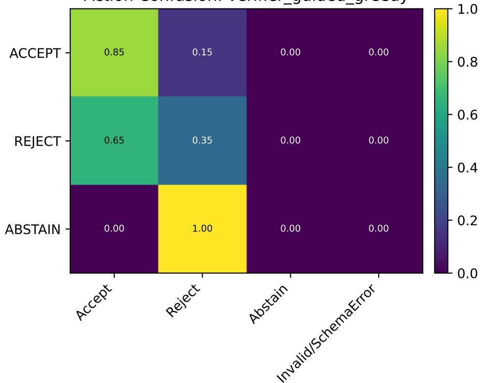
Action Confusion: verifier_guided_greedy
