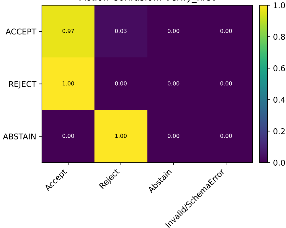
Action Confusion: verify_first
