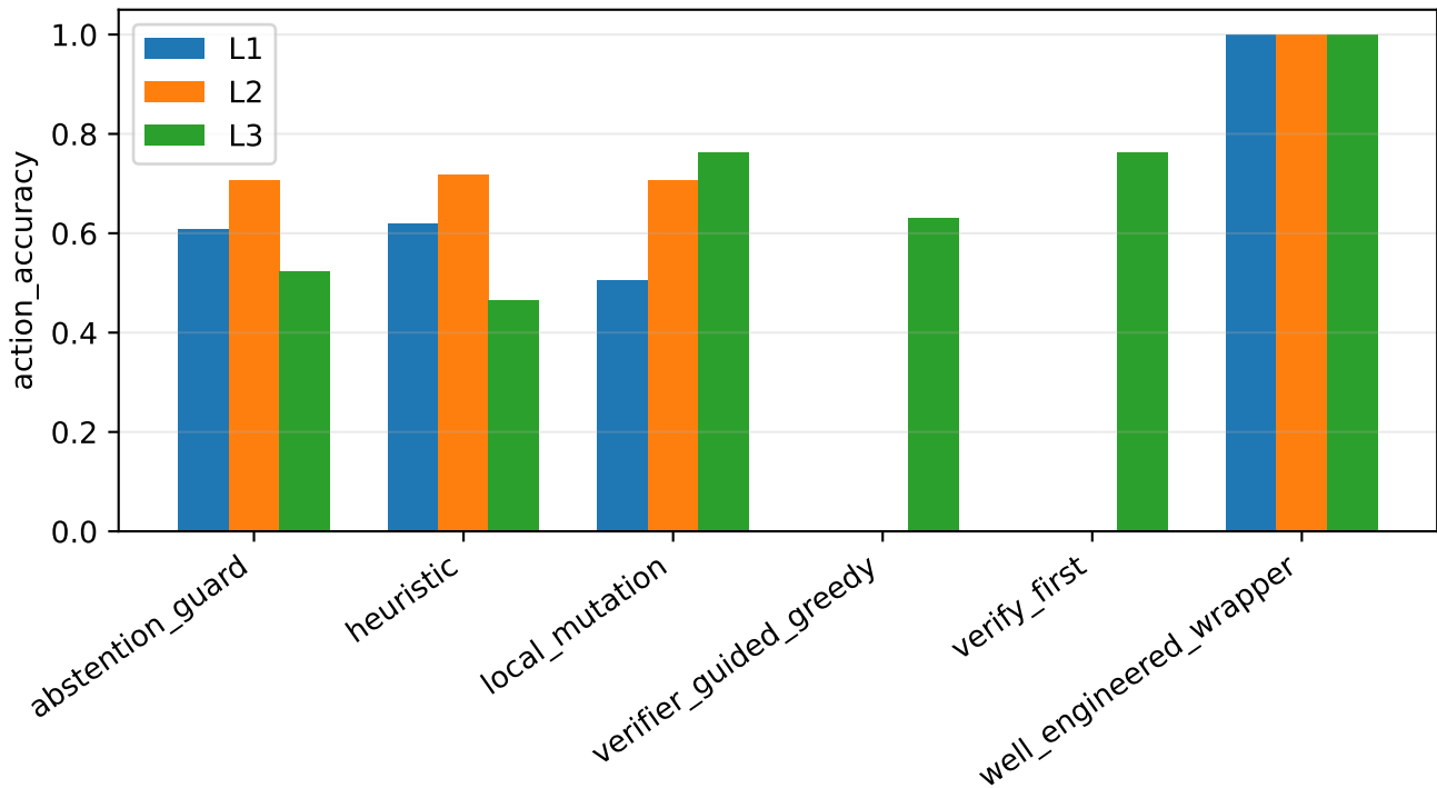
Protocol Ladder Action Accuracy
