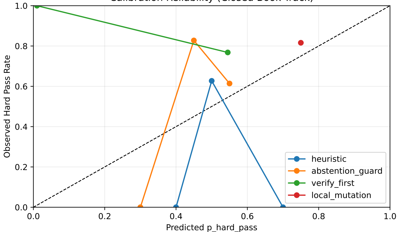
Calibration Reliability (Closed Book Track)
