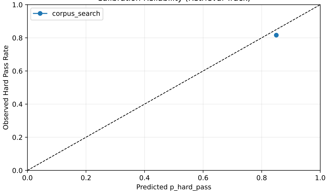
Calibration Reliability (Retrieval Track)
