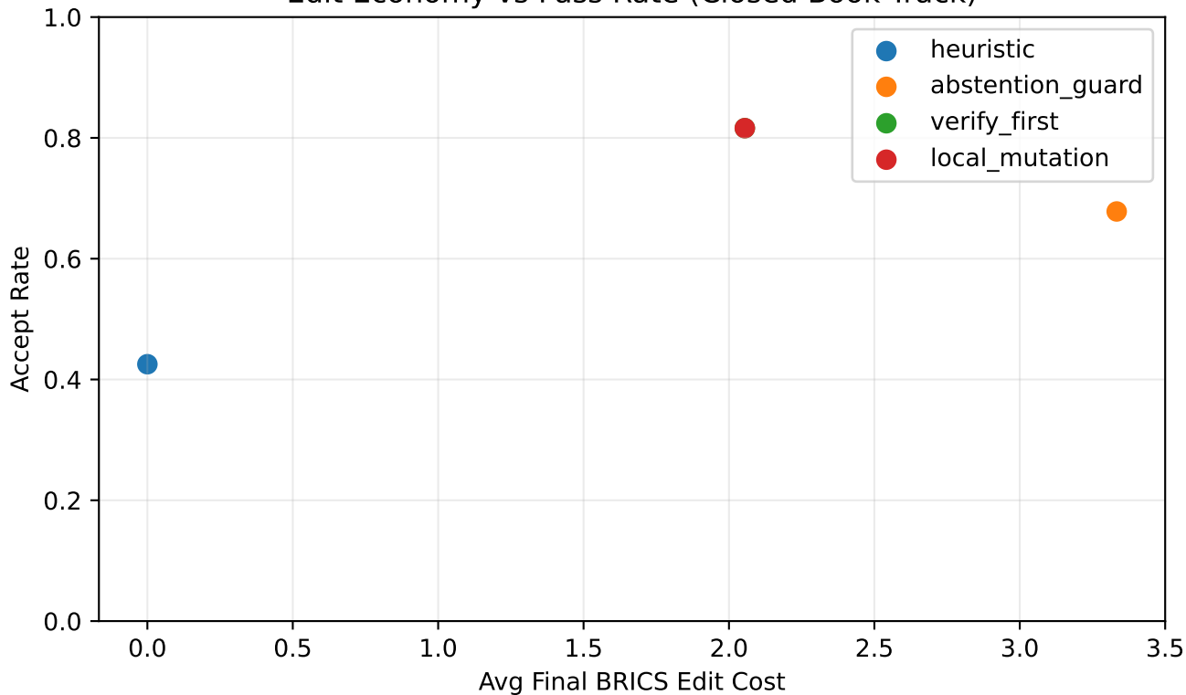
Edit Economy vs Pass Rate (Closed Book Track)
