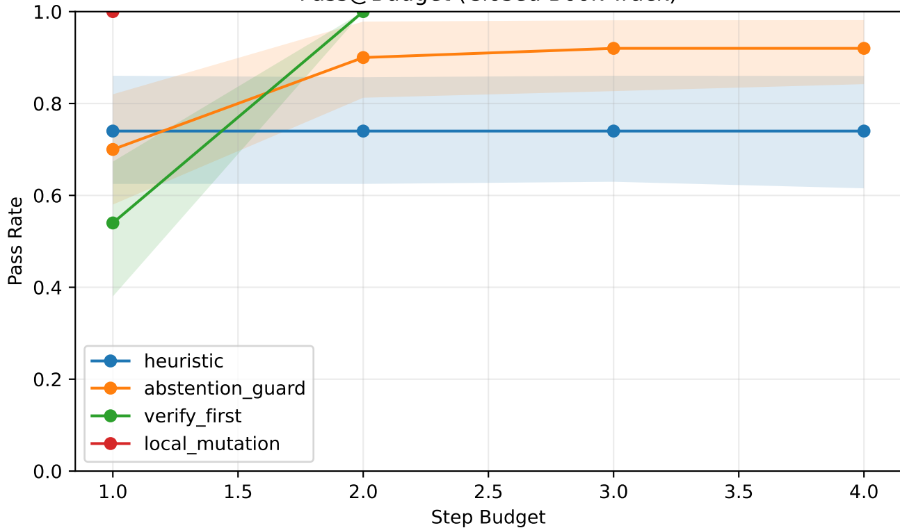
Pass@Budget (Closed Book Track)
