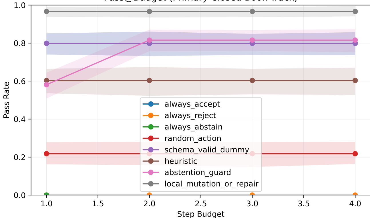
Pass@Budget (Primary Closed Book Track)
