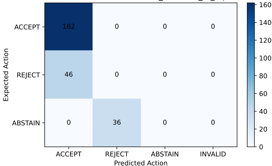
Action Confusion Matrix (local_mutation_or_repair)
