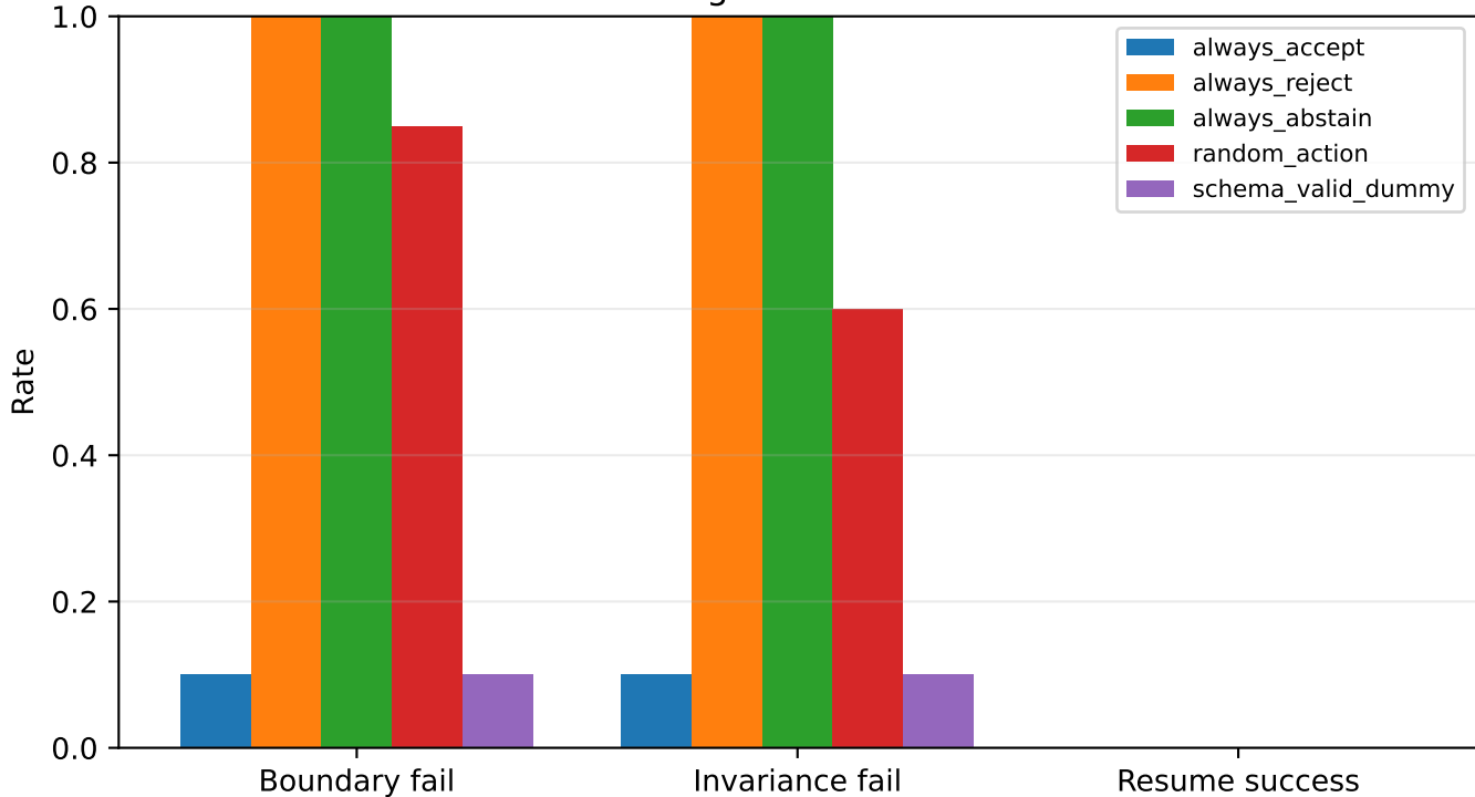
Diagnostic Slices
